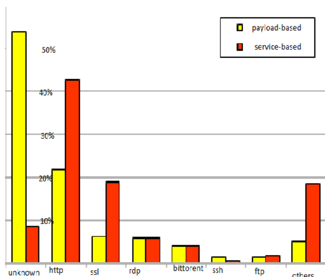
Comparison of both service and payload-based classification
